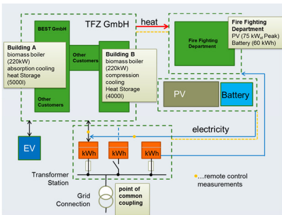
fig. 2) Concept of Microgrid Lab Wieselburg
